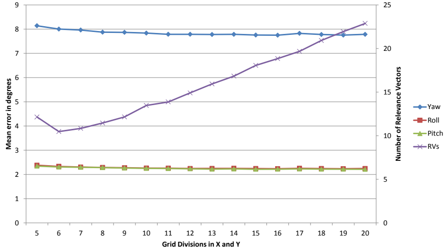
Fig. 4. The effect of varying the grid size used in feature generation, on the average mean error in the three head rotation angles (yaw, pitch, and roll). The grid of size 15 \times 15 yields the best results.
