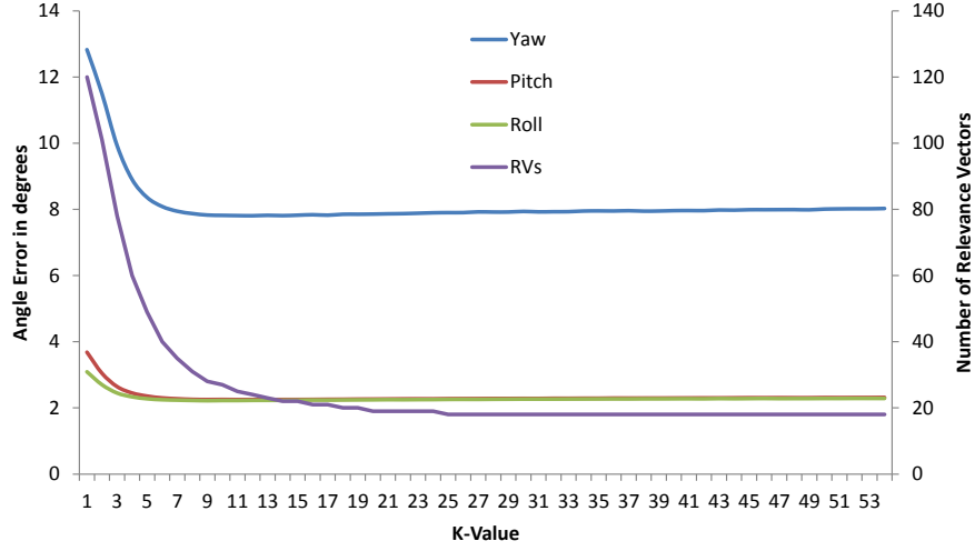
Fig. 3. The effect of varying the kernel width \sigma_k on the average mean error in the three head rotation angles (yaw, pitch, and roll). On the secondary axis, the number of relevance vector is shown.
