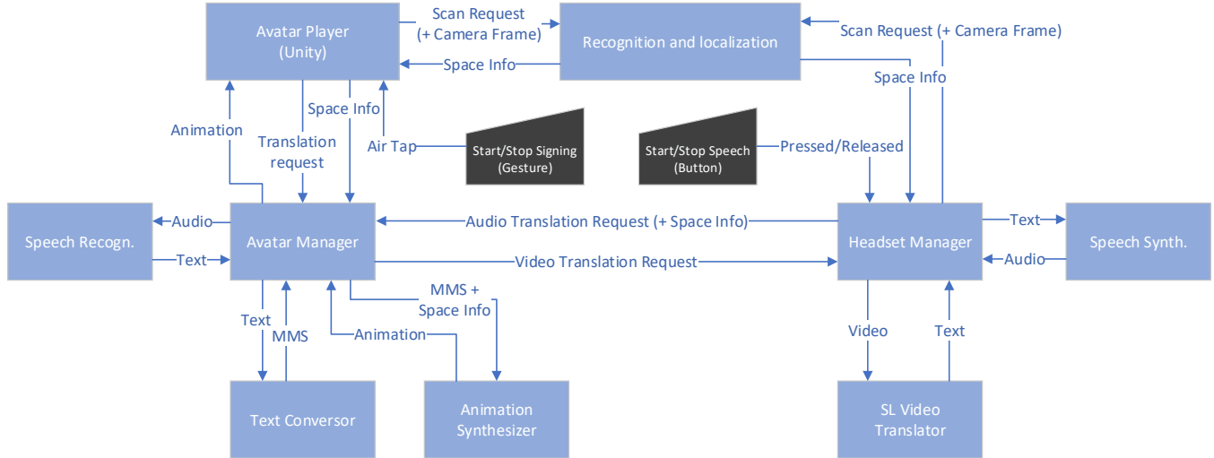
Fig. 2. Component diagram of the proposed application.
