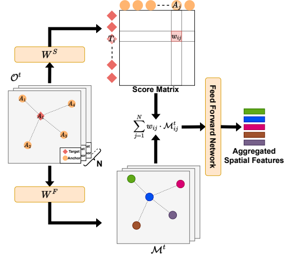
Figure 4. Our novel attention-based spatial feature aggregation. Each map designates a different object as the target, while treating all other objects as anchors. The importance of each anchor relative to the potential target object is represented in row i of the score matrix, indicating the relevance of each anchor in the context of the target, where W_S and W_F are learnable weight matrices.
