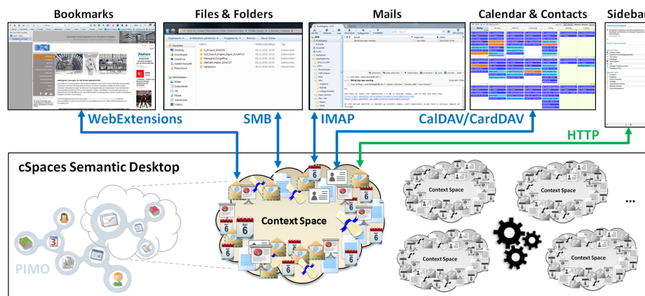
Fig. 1. Conceptual overview of the cSpaces Semantic Desktop
